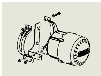
Drawing of RB-DUR19
