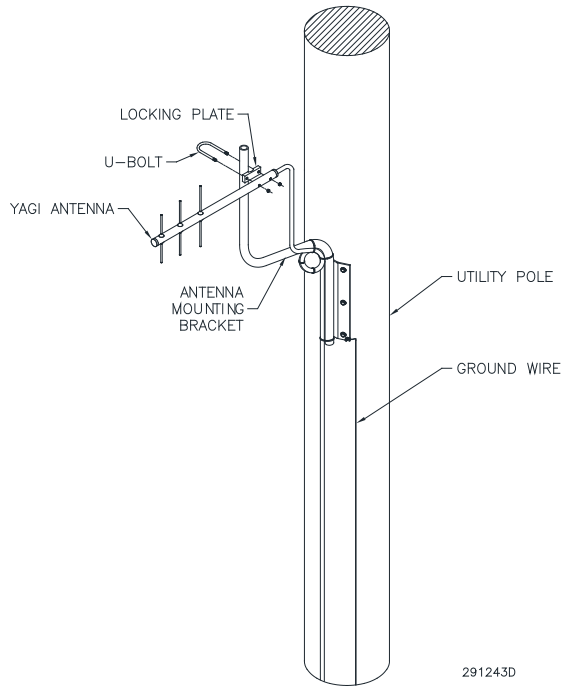
Figure 1 Yagi Antenna Installation Example
