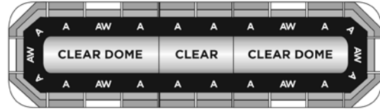
ALGT53D-AMBR1FC 53", Amber, takedowns, alley lights, work lights, flat mount, Clear domes ALGT53D-AMBR1HC 53", Amber, takedowns, alley lights, work lights, hook mount, Clear domes
