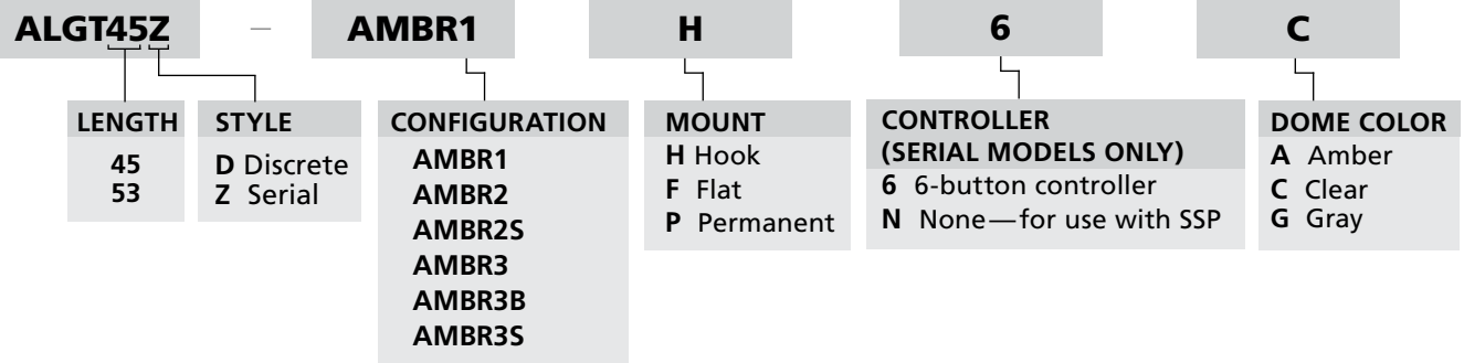
AMBR1 Amber, (2) LED takedowns, (2) LED alley lights, (2) LED work lights (SignalMaster in Serial only)
