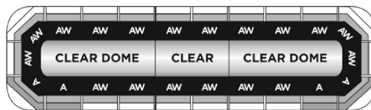
ALGT53Z-AMBR3F6C 53", Amber, front and rear flood, SignalMaster, flat mount, 6-button controller, Clear domes ALGT53Z-AMBR3H6C 53", Amber, front and rear flood, SignalMaster, hook mount, 6-button controller, Clear domes
