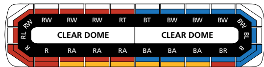
RLNT48-P3LC (without interface module, low hook mount)
