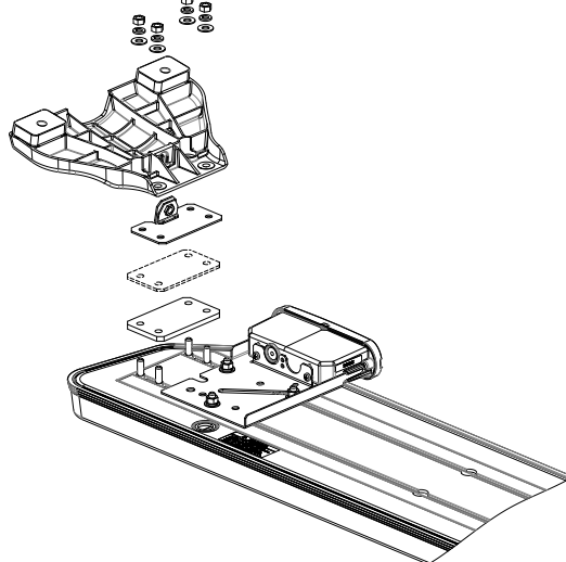
Figure 1 Position of shim (passenger side)
