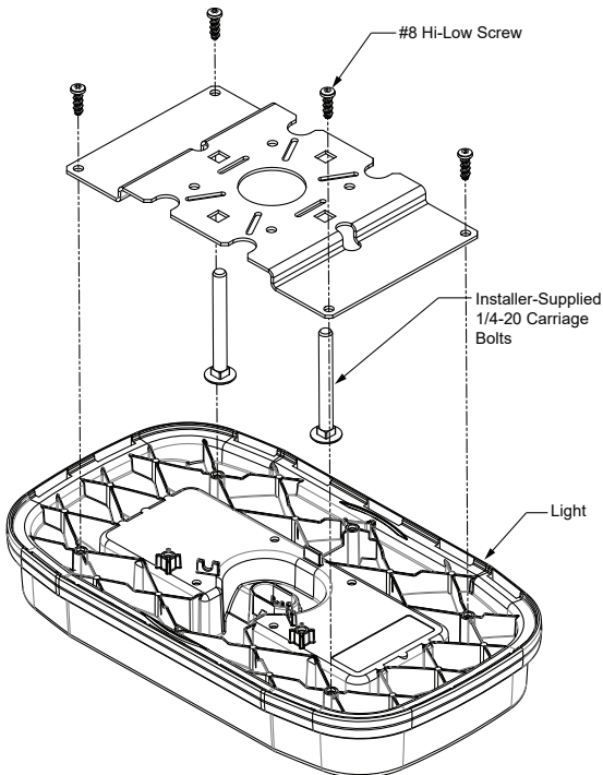
Figure 3 Bar Mount
