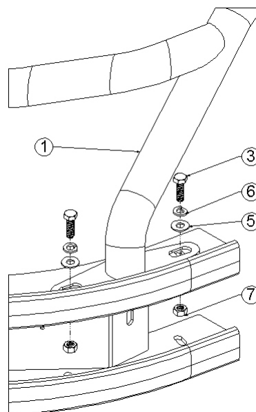
Figure 3 Attach upper guard to lower guard
