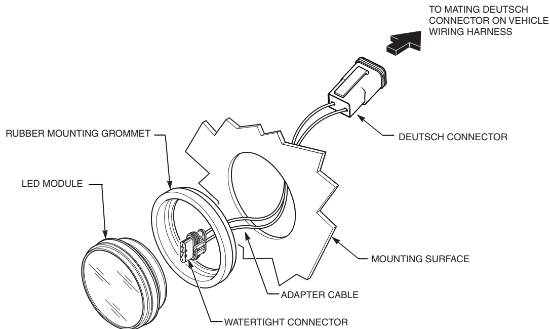
Figure 1: Connection between LED module and vehicle wiring harness
