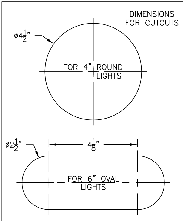
Figure 1 Dimensions for cutouts
