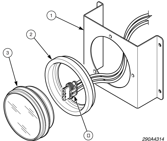
Figure 2 Exploded view of light installation
