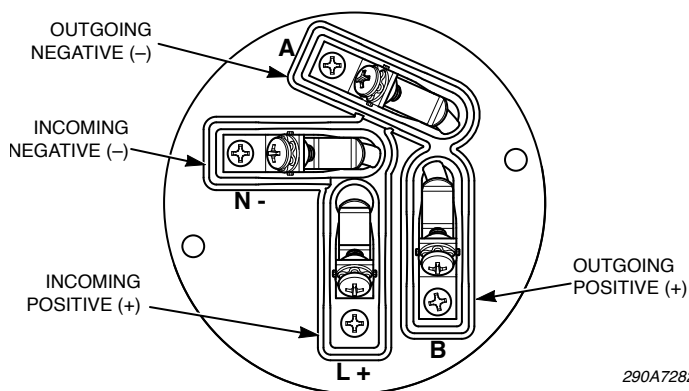
Figure 3 Terminal block
