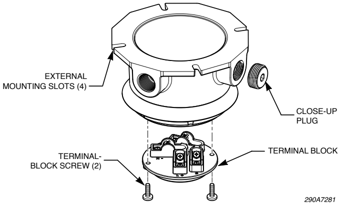
Figure 2 Exploded view of light
