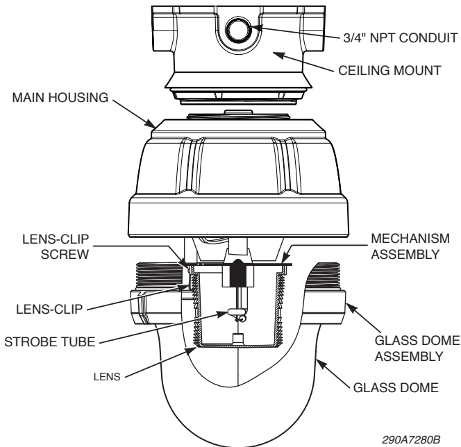
Figure 2 Exploded view of light
