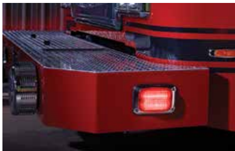
FireRay LED 6x4 (FR6C-R) mounted on bumper with two-to-four hole conversion kit (FR6-A4HMC)
