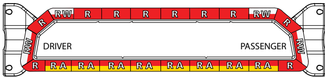
INTG44J-F1H (hook mount)
