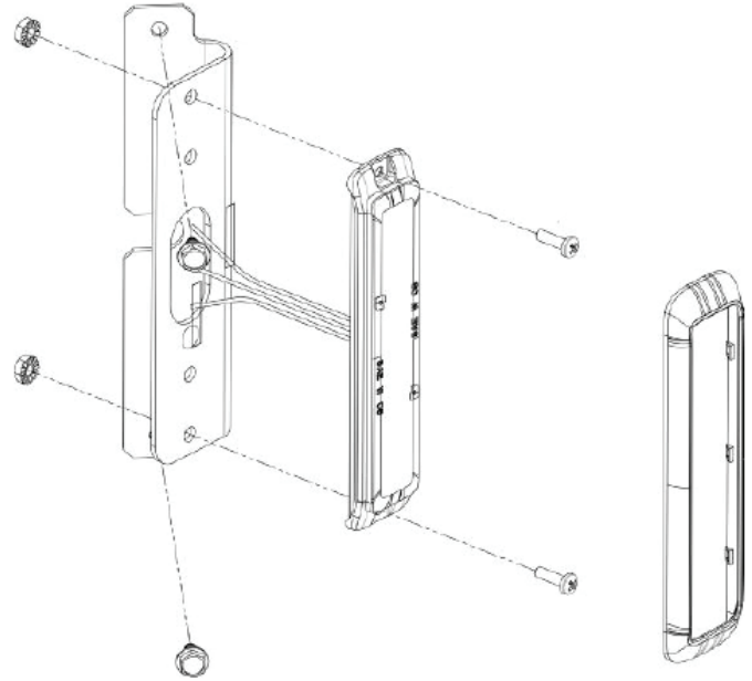
Drawing of MPSU-PB45V
