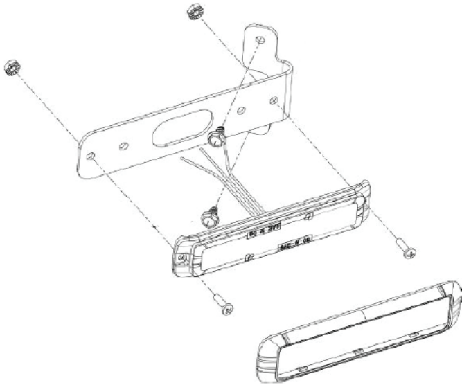
Drawing of MPSU-PB45H
