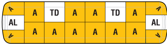
LGD45Z-AMBR2H6 45", Amber, Takedowns, Alley lights, Hook Mount, Clear Domes, Six-button Controller
