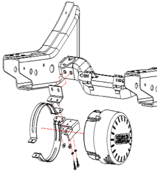
Front of bumper with RUMBLER-3 siren
