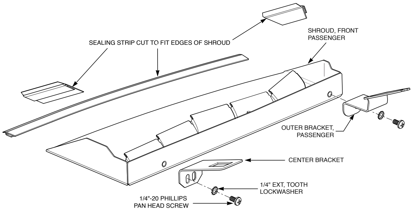
Figure 1 ILS installed with mounting system on passenger-side
