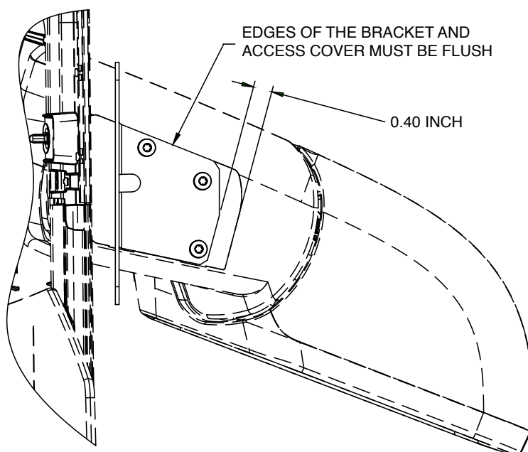
Figure 1 Passenger-side bracket secured on mirror access cover
