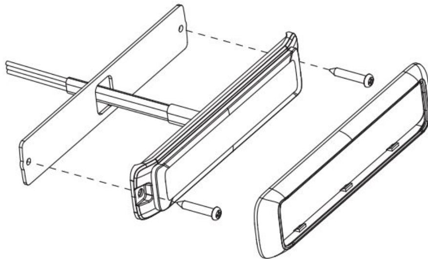
Figure 1 Exploded view
