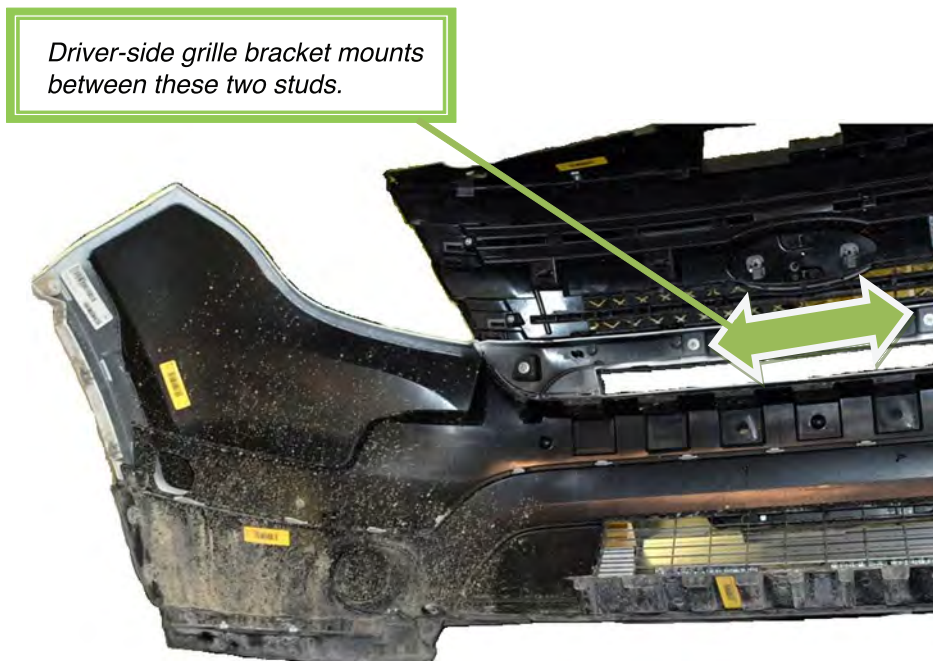
Figure 3 Mounting location of driver-side grille bracket
