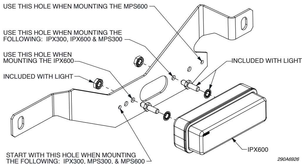
Figure 1 Lighthouse mounting configurations
