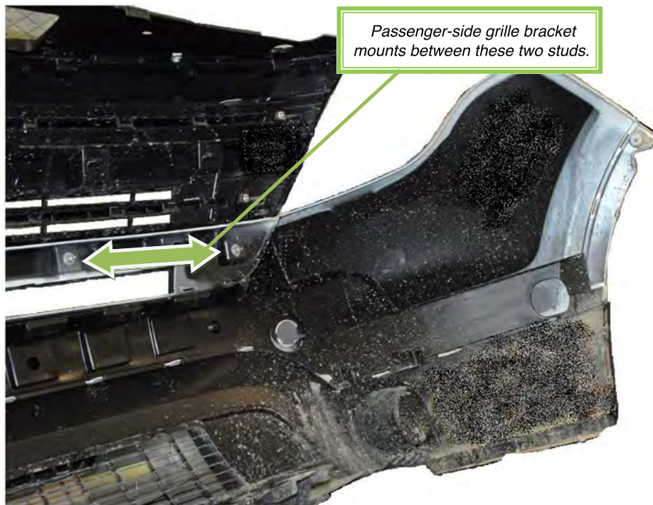
Figure 2 Mounting location of passenger-side grille bracket
