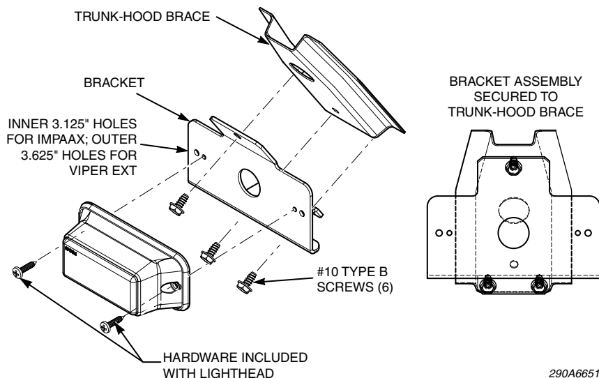
Figure 1 Lighthead with bracket attached to trunk brace
