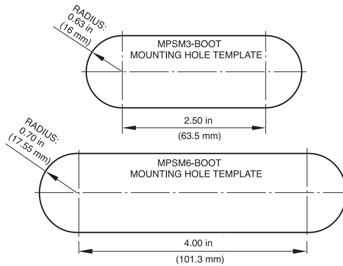
Figure 1 Mounting holes for MPS300 and MPS600 with boot
