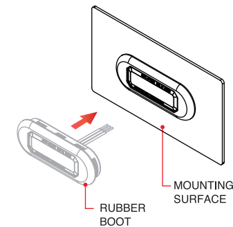
Figure 3 Lighthouse with boot inserted in mounting hole
