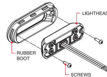
Figure 2 Lighthouse secured in boot with hardware
