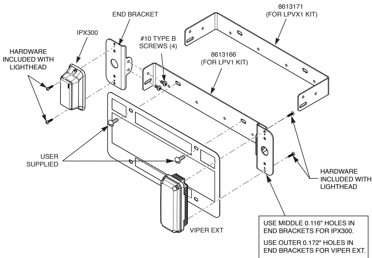
Figure 1 IPX300 and Viper EXT mounted to center bracket
