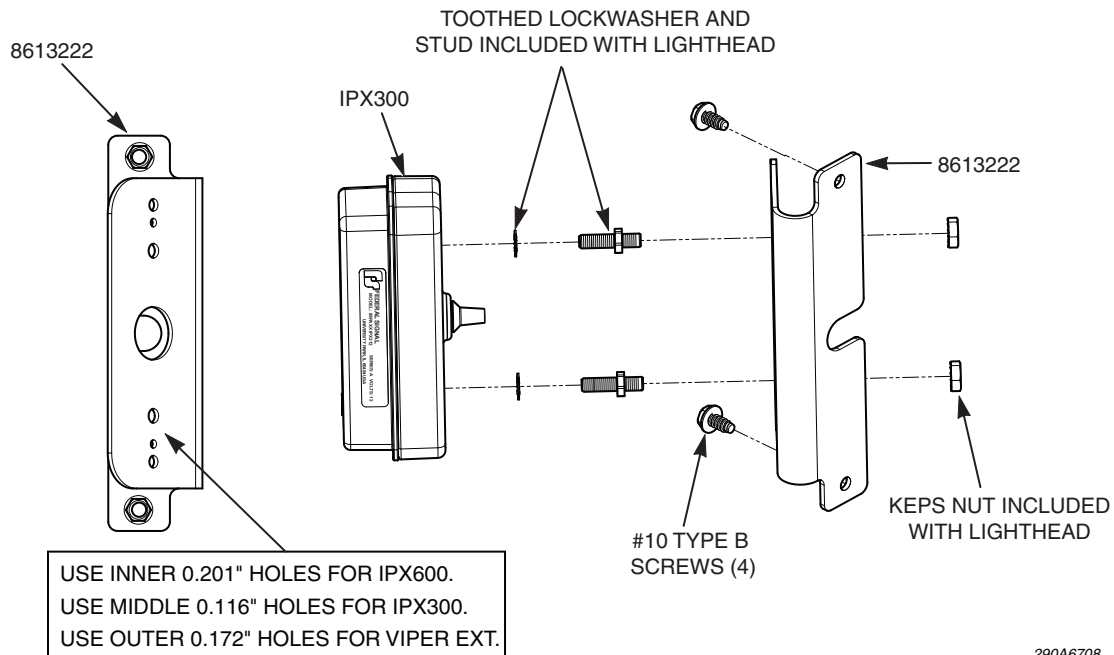
Figure 1 IPX600 lighthead attached to canter bracket with end bracket
