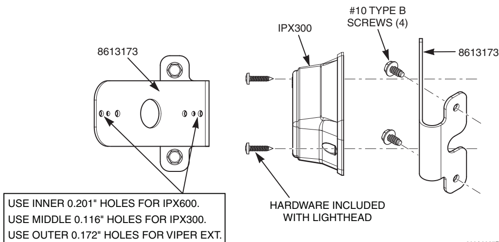
Figure 1 IPX300 lighthouse attached to horizontal bracket
