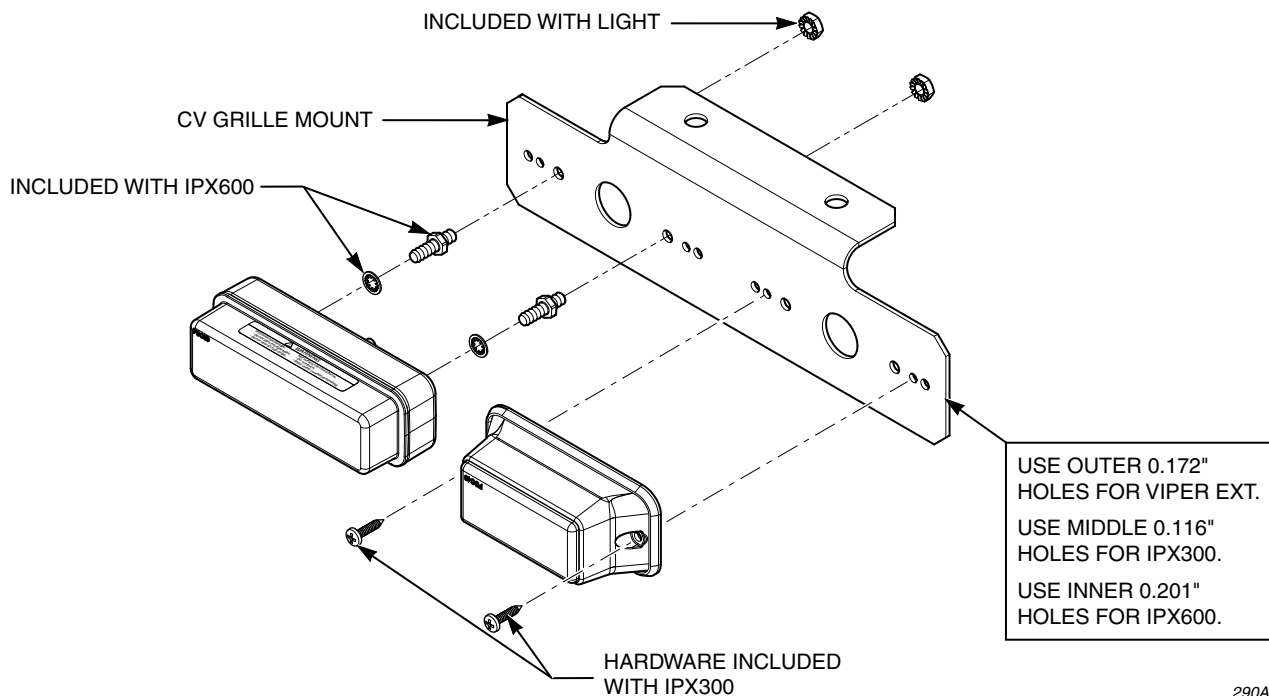
Figure 3 IPX600 lights secured to bracket
