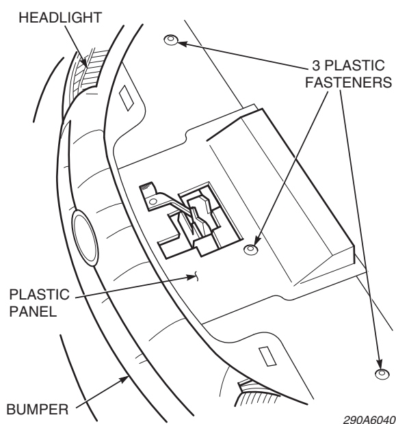
Figure 1 Remove the plastic panel to install bracket
