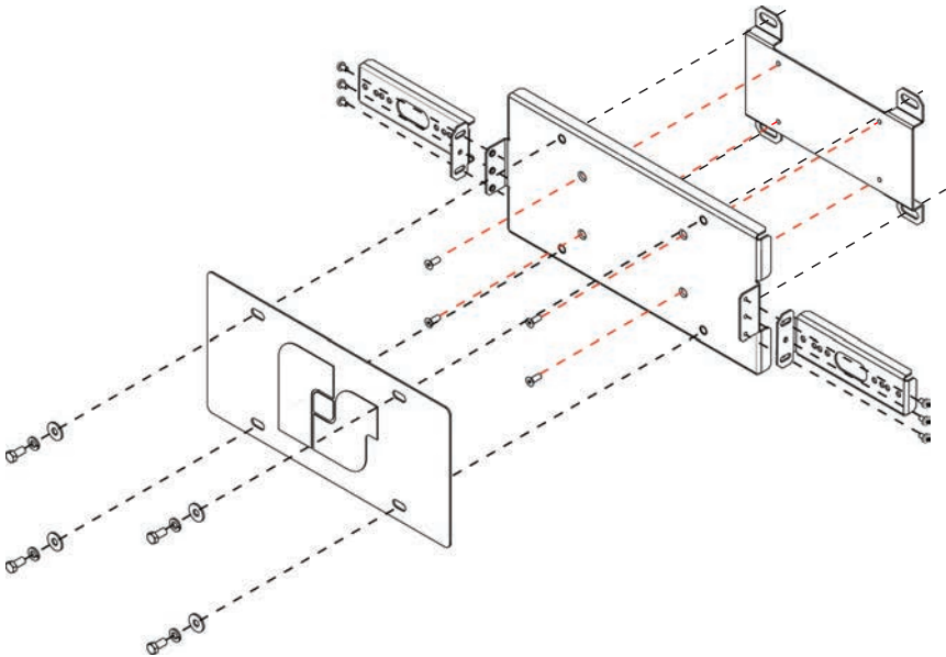
Figure 1 Exploded View
