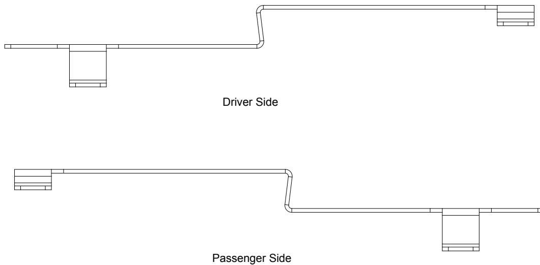
Figure 2 Bracket identification
