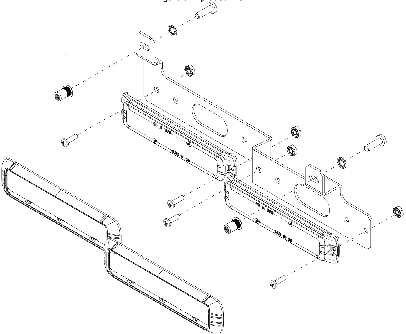
Figure 3 Exploded View
