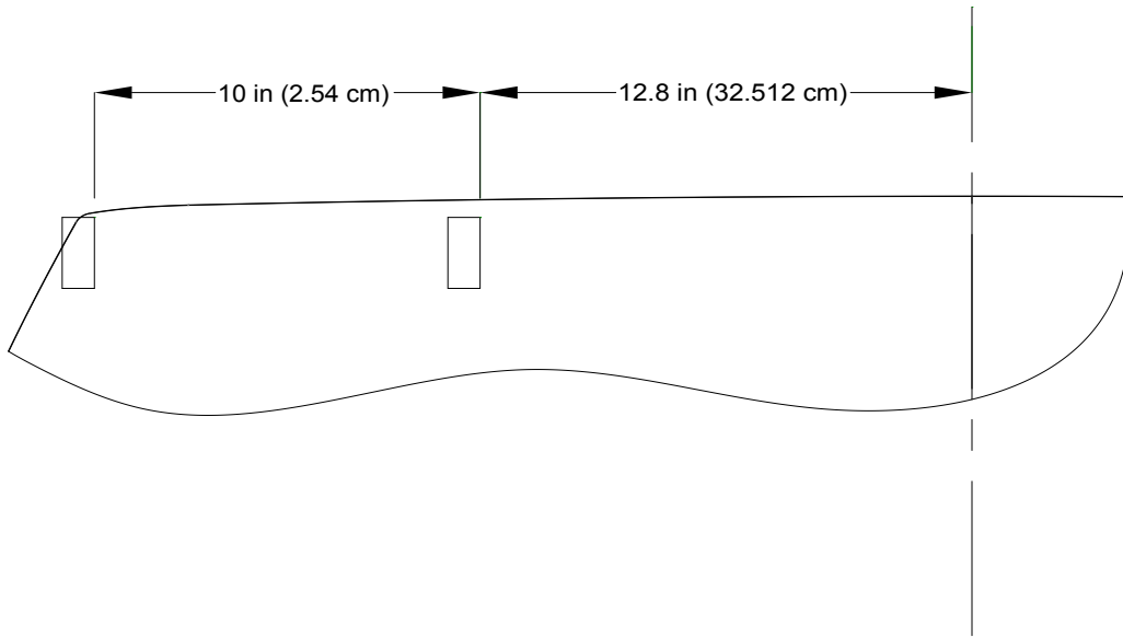
Figure 4 Mount gasket to the back glass
