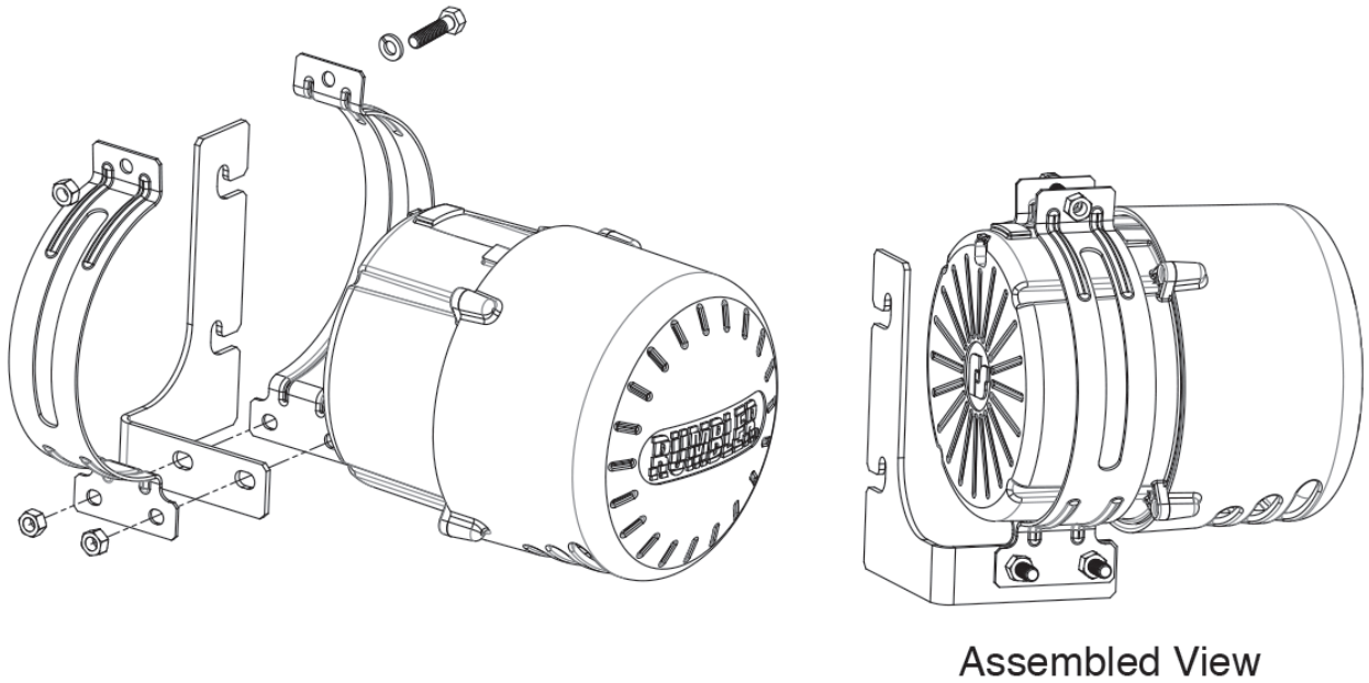
Figure 3 Rumbler Installed
