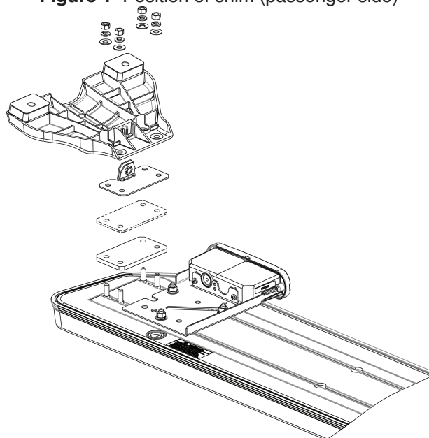
Figure 1 Position of shim (passenger side)
