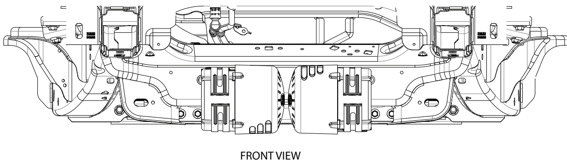
Figure 3 Rumlbers and brackets installed on frame of F-150
