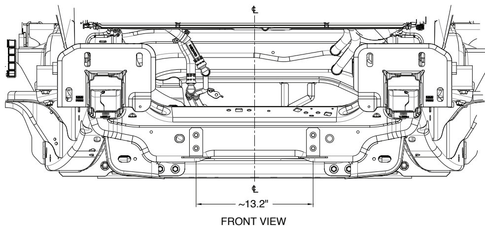
Figure 1 Rumbler brackets installed on frame of F-150
