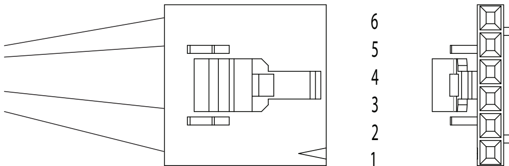
Figure 1 Cable 17501771 Pinouts
