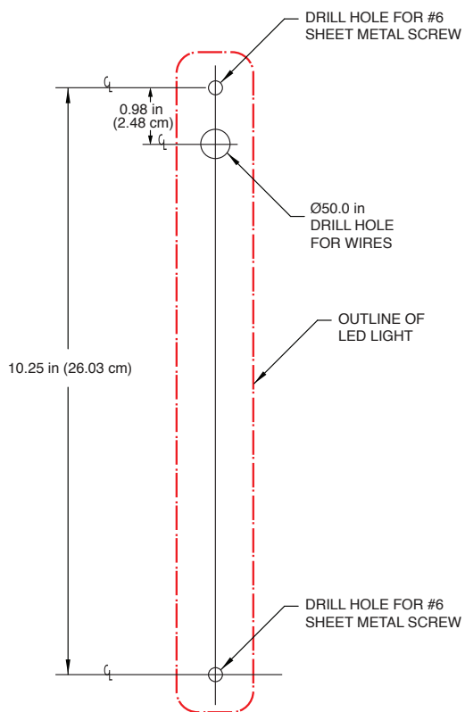
Mounting holes and dimensions (not to scale)
