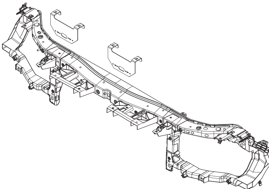
Figure 1 Brackets positioned over mounting holes in support
