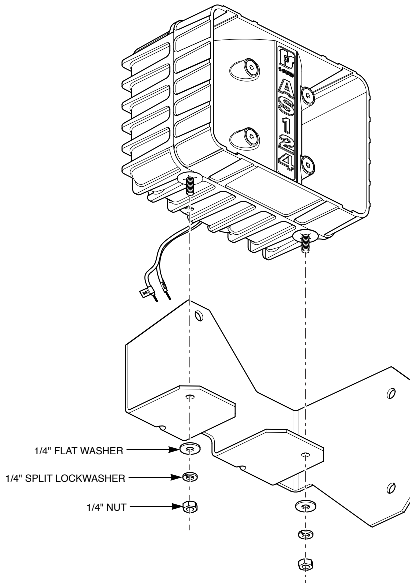
Figure 2 AS124 and bracket with mounting hardware supplied with speaker
