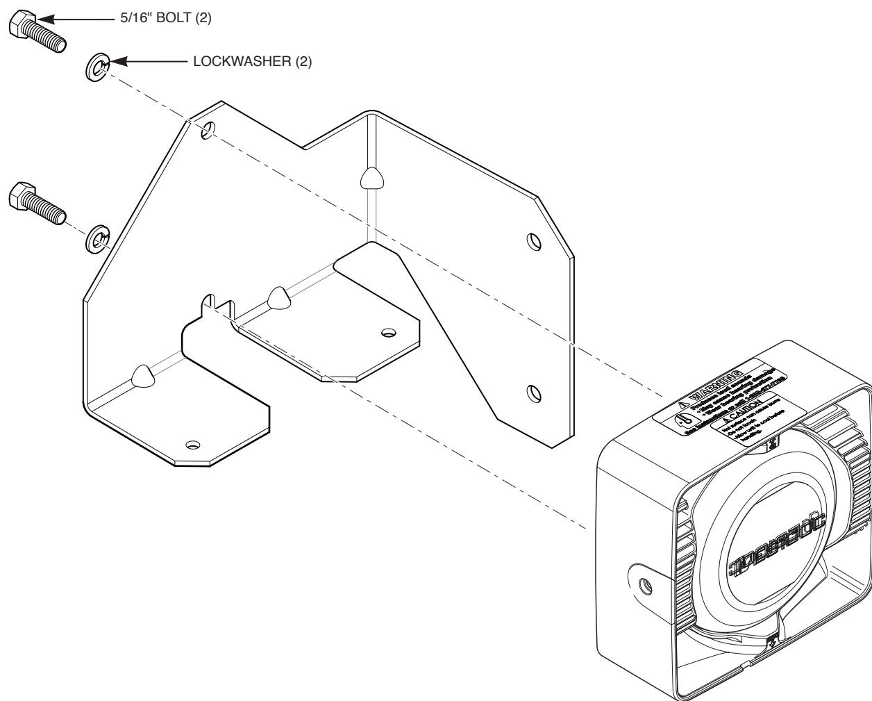
Figure 2 ES100C and bracket with mounting hardware supplied in kit
