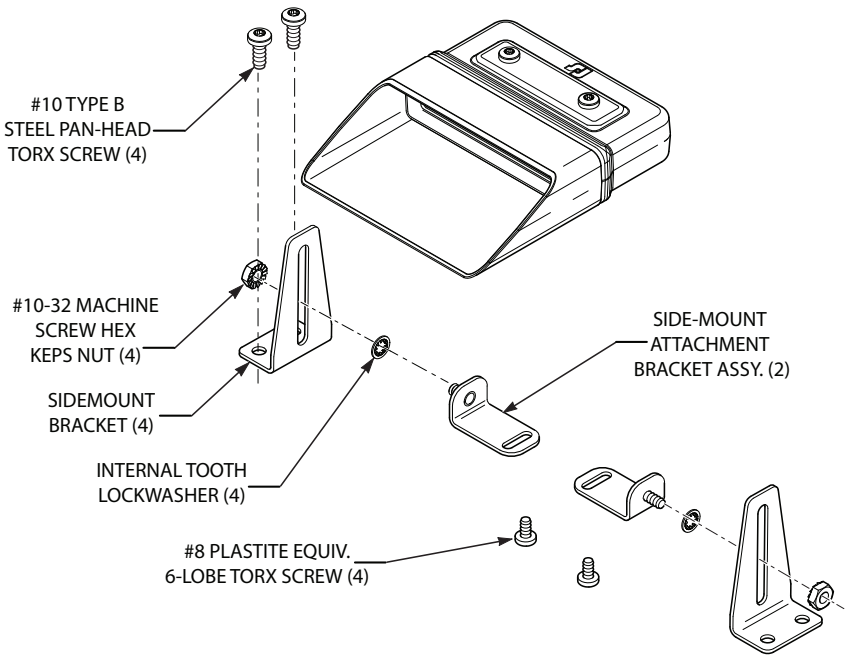
Figure 1 Exploded view of lighthouse with mounting brackets
