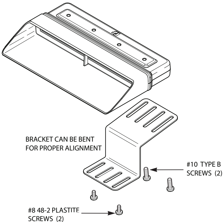
Figure 1 Light attached through headliner
