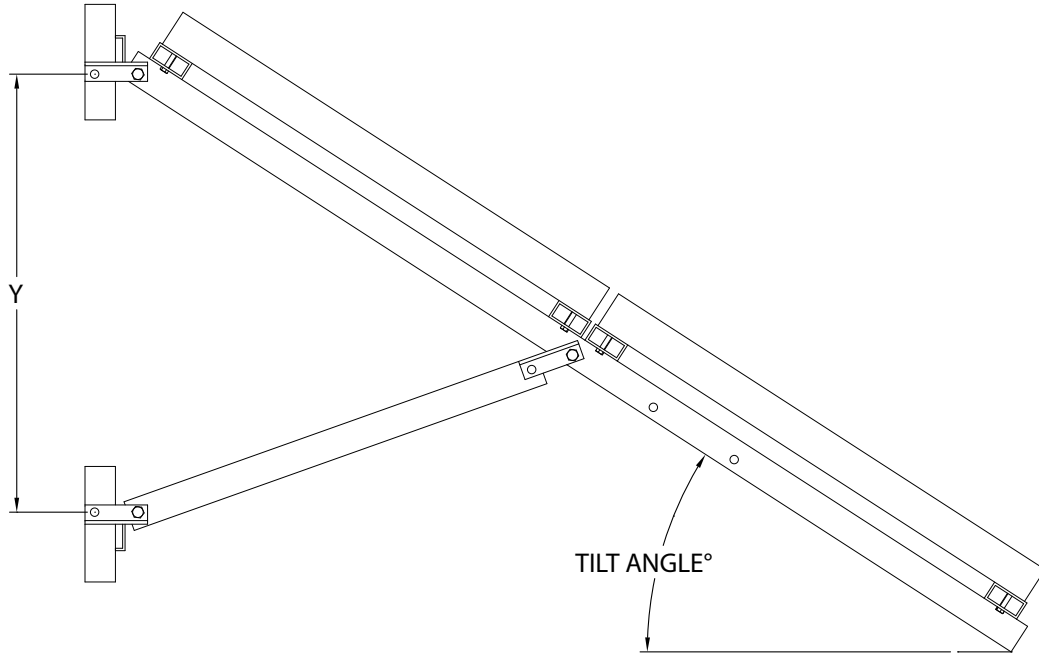
Figure 2 Side Pole Mount (65+ W Modules)
