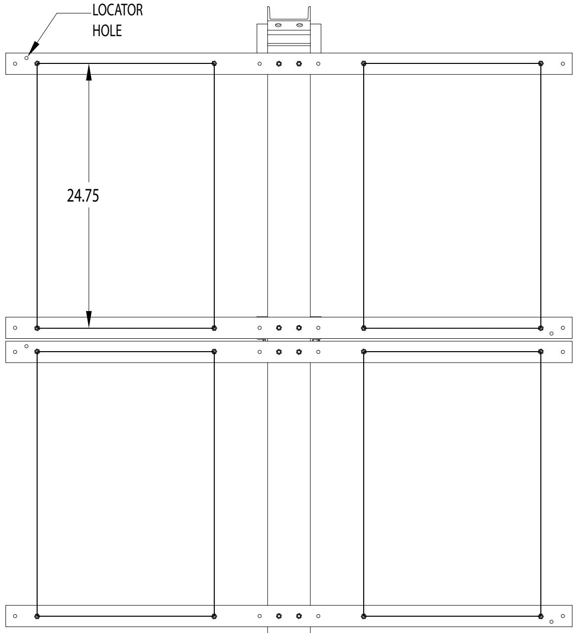
Figure 1 Placement of 65+ W Module (Top View)
