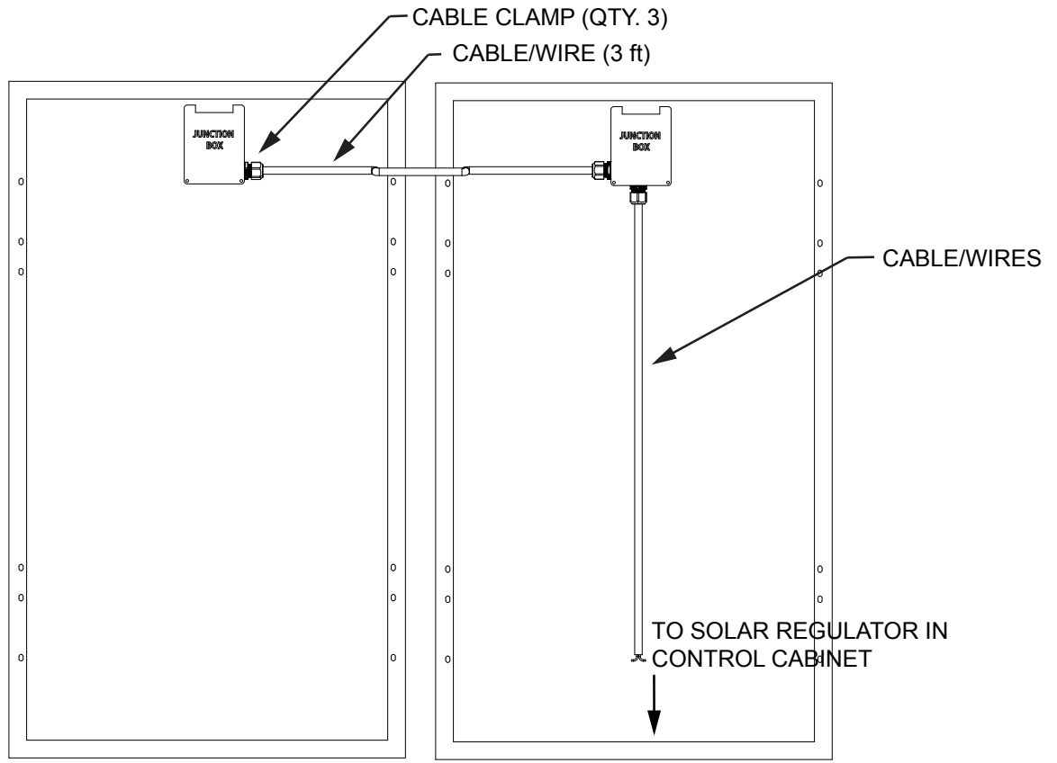
(BACK VIEW) MODULE WIRING 110 W PANELS
