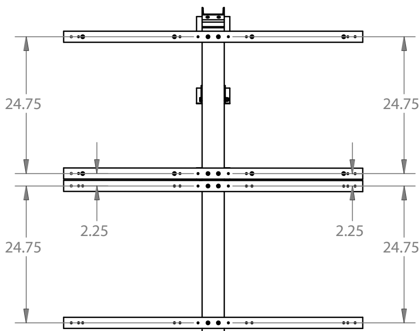
BRACKET ASSEMBLY
