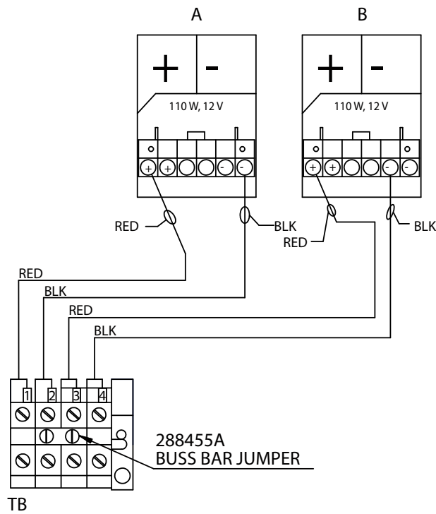
24 V HAWAII VERSION WIRING
