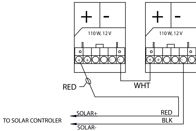
24 V STANDARD VERSION WIRING
