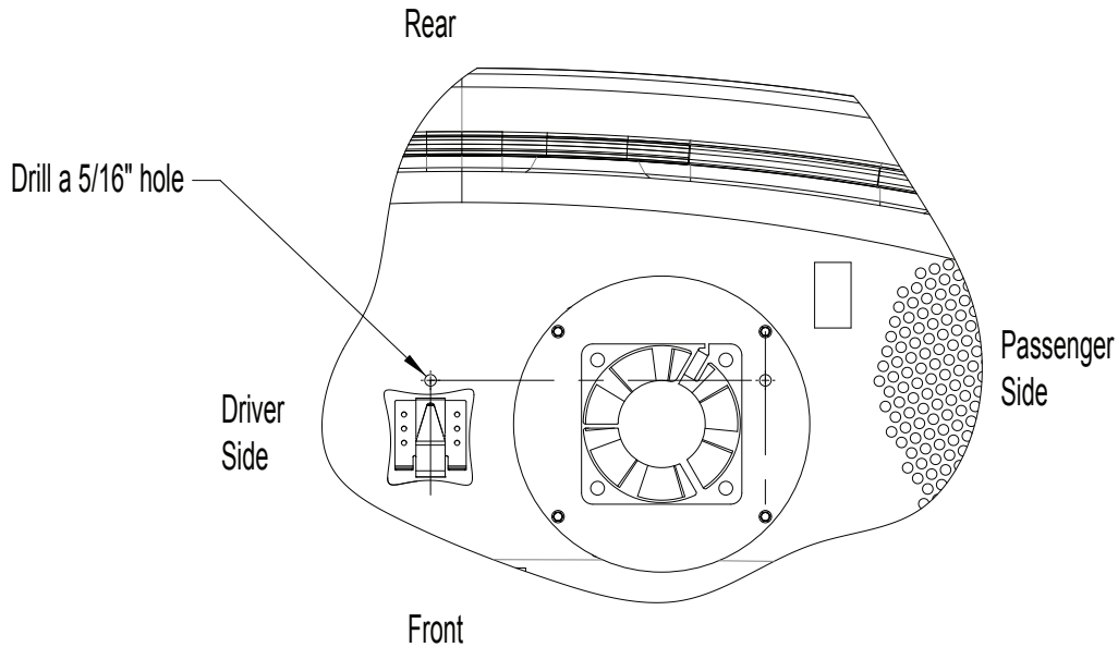
Figure 2 Location of drilled holes in underside of package tray 2017 Charger
