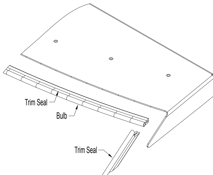
Figure 1 Install the trim seal
