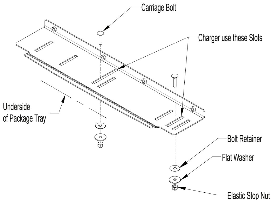
Figure 3 Hardware securing baseplate to rear deck
