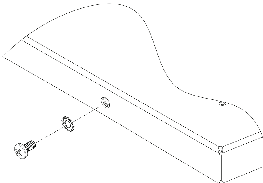
Figure 4 Attach the shroud
