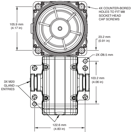
Figure 5 Front view of Ex de surface mount
