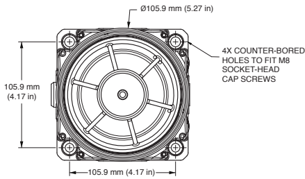
Figure 2 Front view of Ex d beacon
