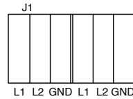
Figure 9 IN/OUT PCB connections for Ex d 120-240 Vac
