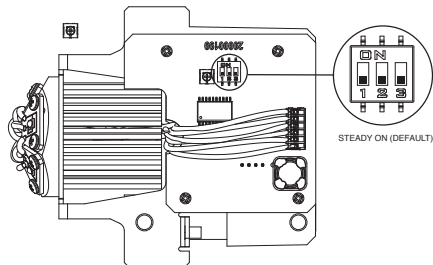
Figure 11 Location of DIP switch for flash patterns
