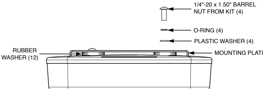
Figure 1 Mounting bracket attached to the lightbar
