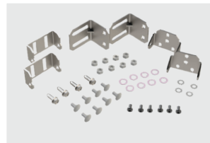
CNSM-UM Universal mount for internal/external use
