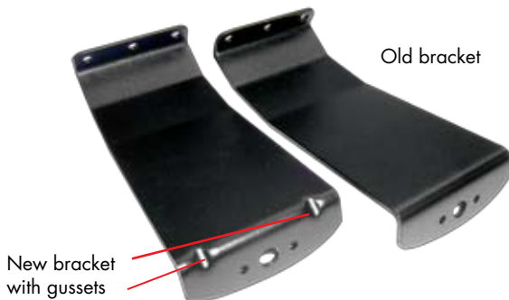
Hook kits have been gusseted to improve strength
