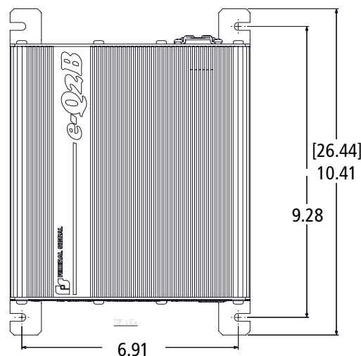
Mounting Dimensions
