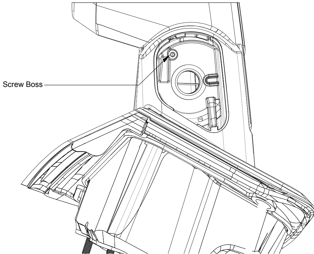
Figure 2 Screw Boss
