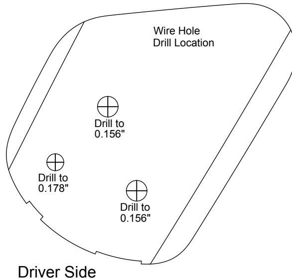
Figure 1 Drilling Template
