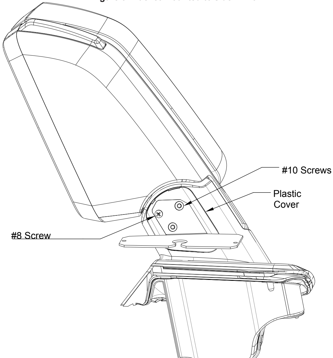
Figure 3 Bracket mounted to side mirror
