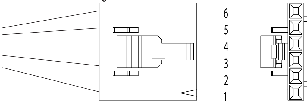
Figure 1 Cable 17501771 Pinouts
