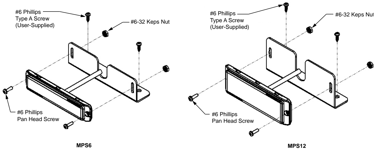
Figure 1 Exploded View
