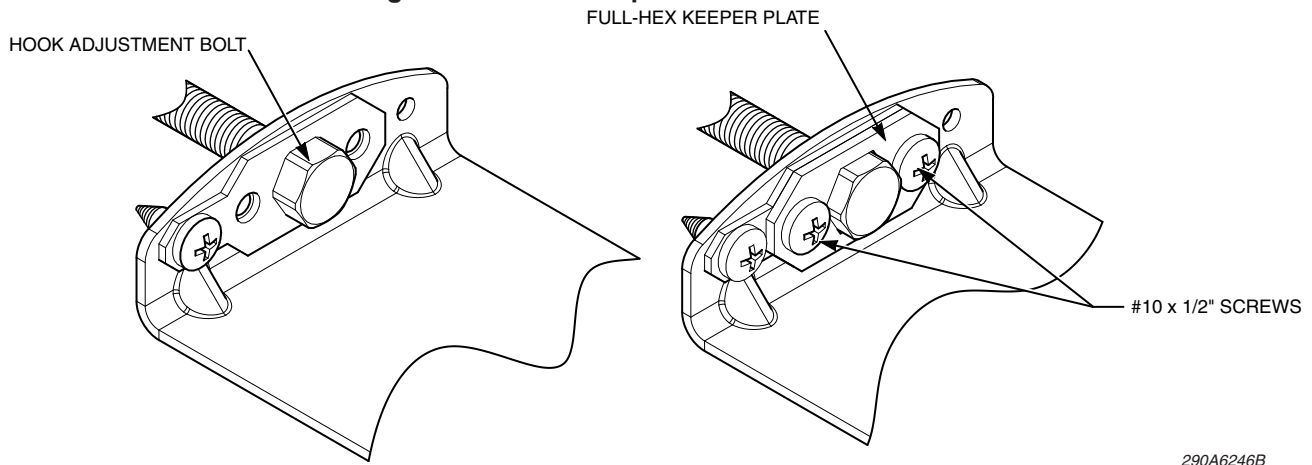
Figure 2 Full-Hex Keeper Plate secured to hook
