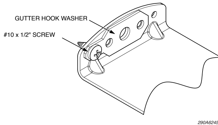
Figure 1 Gutter hook washer attached to mounting hook
