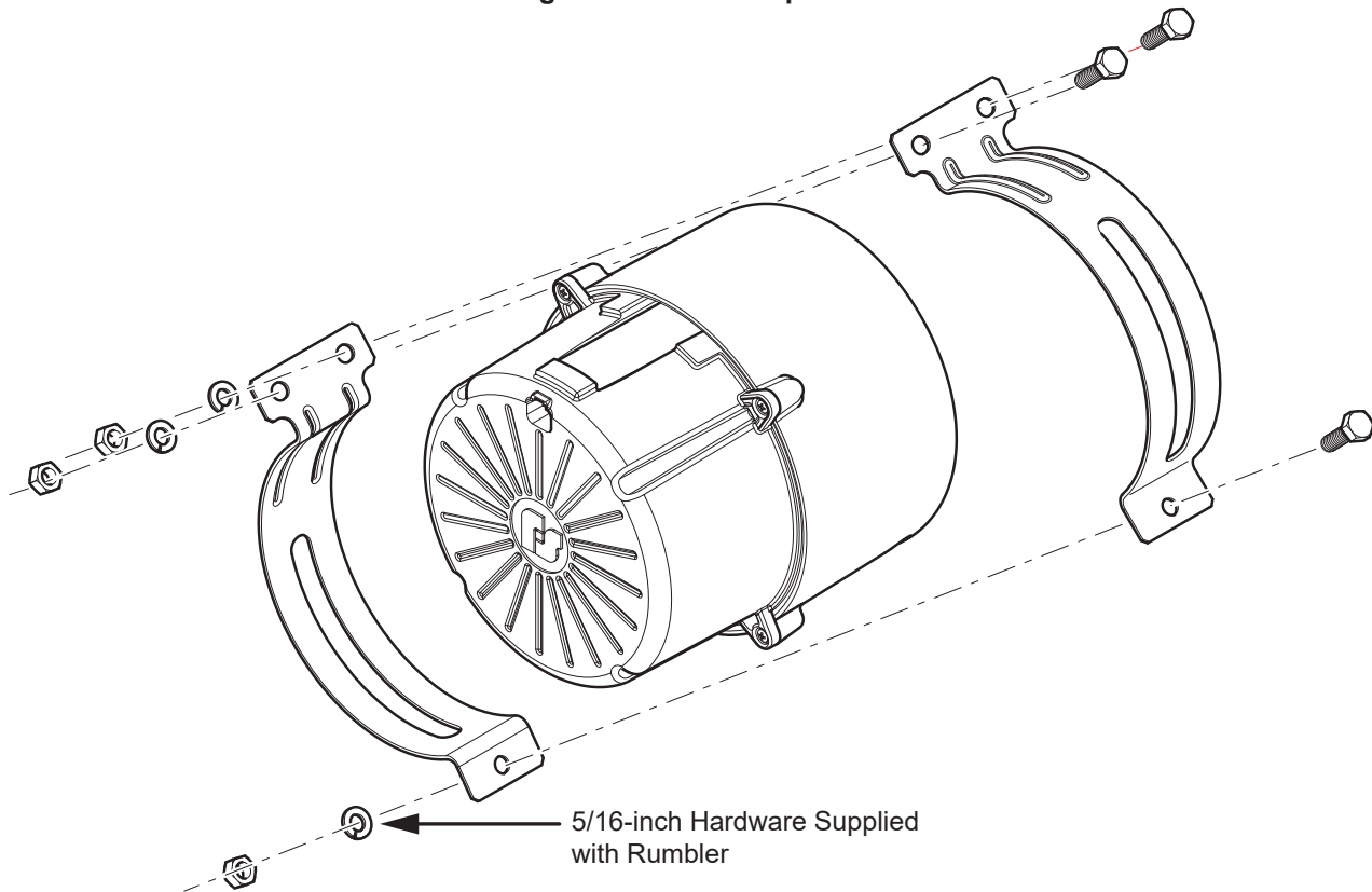
Figure 3 Rumbler exploded view
