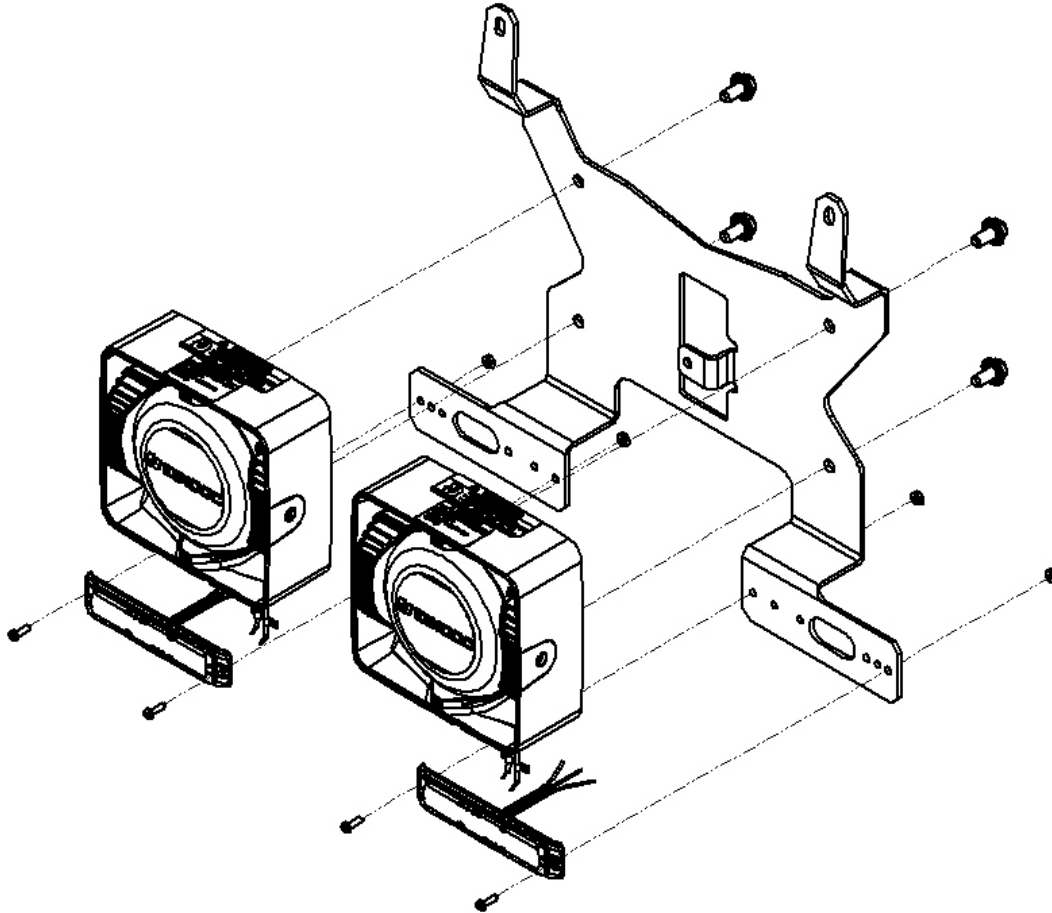
Figure 2 ESBL-SIL22ND Bracket (Dual speaker installation shown)
