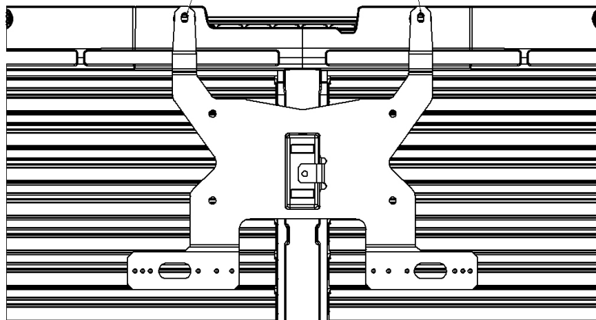
Figure 1 Insert Bracket Assembly BOLT LOCATIONS
