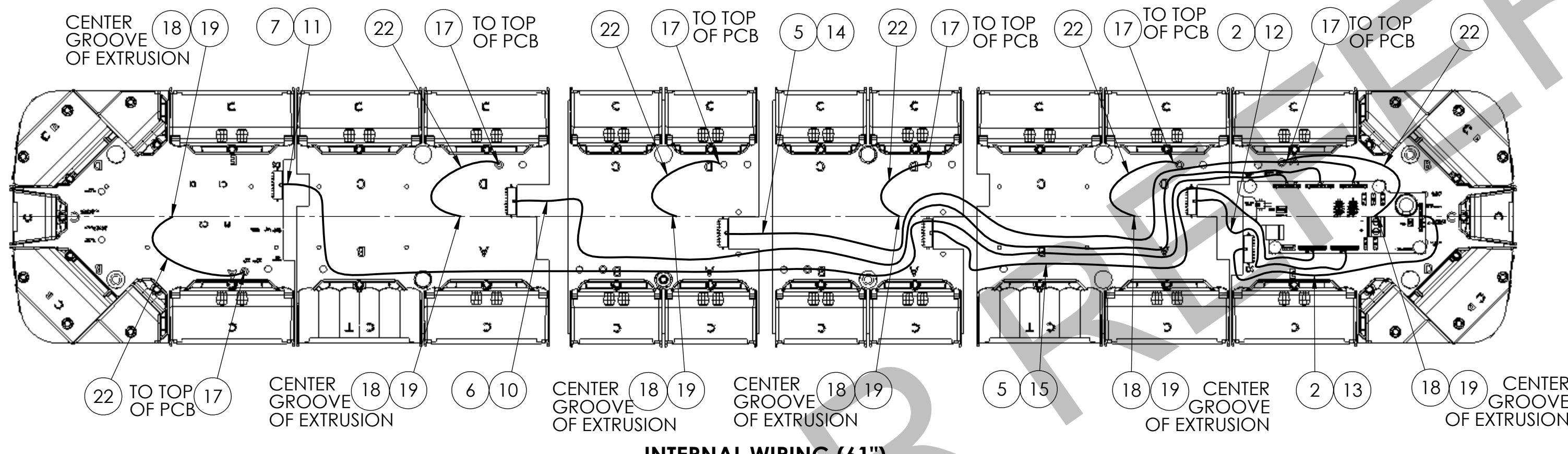
INTERNAL WIRING (61'')
