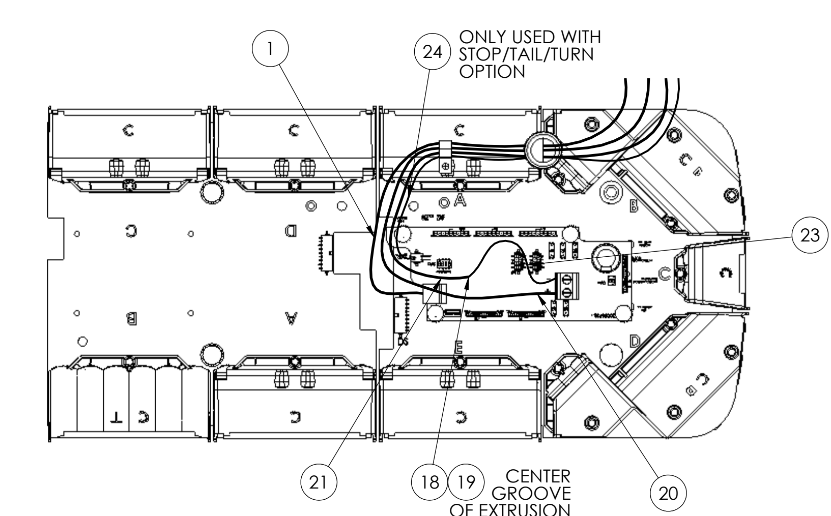
EXTERNAL WIRING (ALL-STD RH CABLE EXIT)
