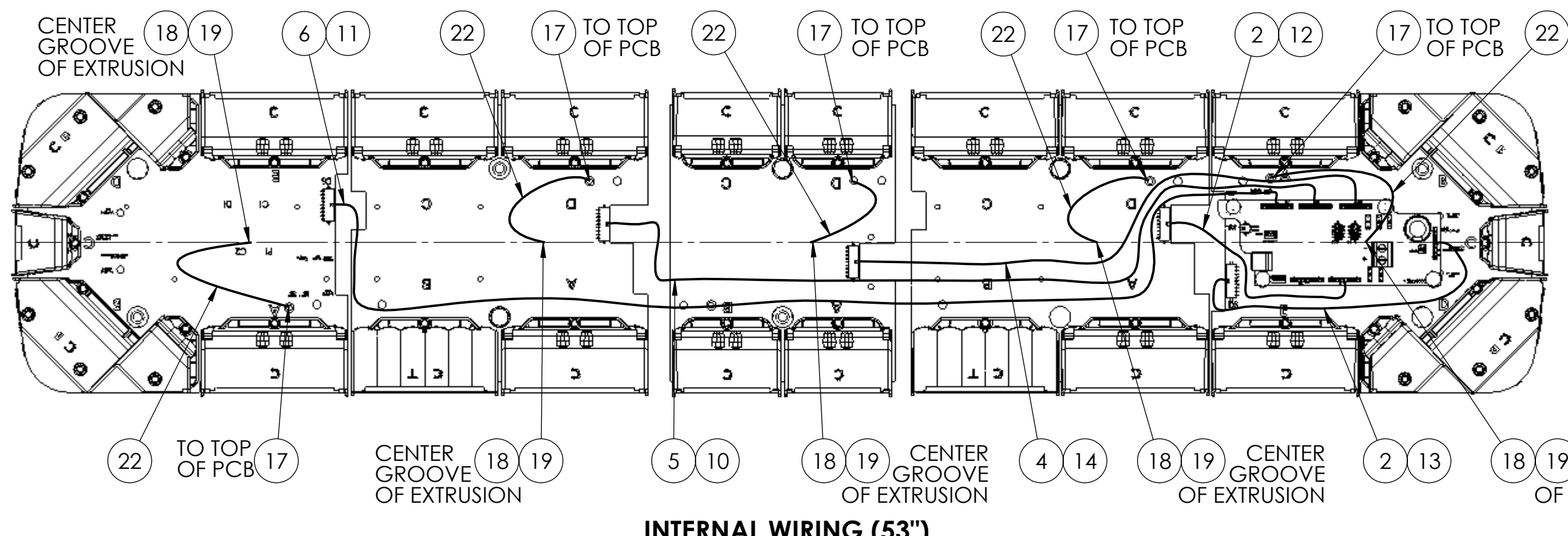
INTERNAL WIRING (53'')
