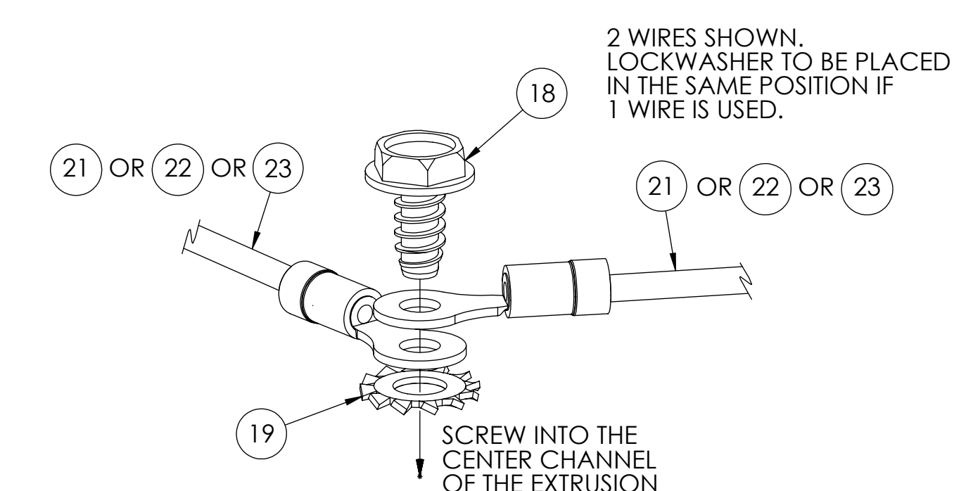
TYPICAL GROUND WIRE CONFIGURATION
